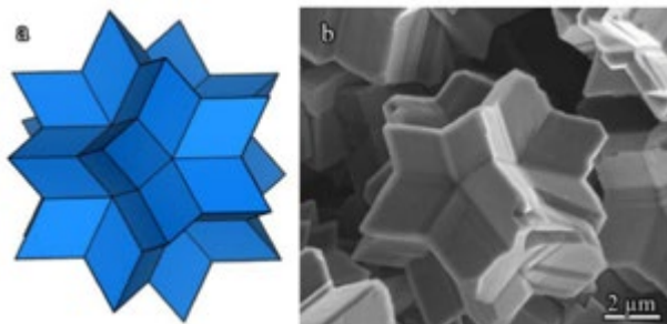
Fig. 1. Rhombic hexecontahedron (a) and scanning electron microscopy image of a particle of boron carbide with the same shape (b).
