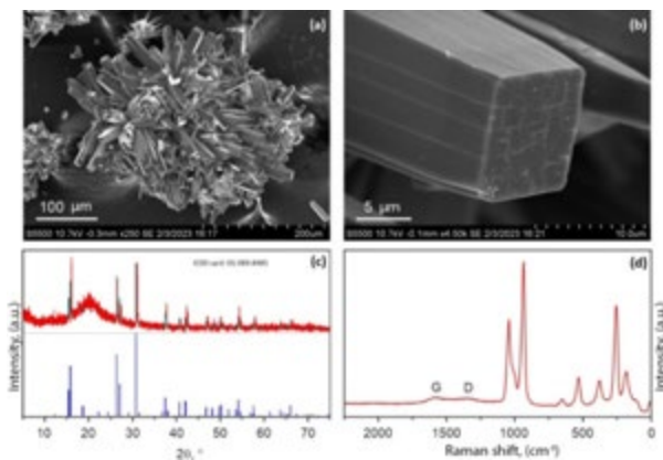
Fig. 1. SEM images of particle surface (a, b), X-ray pattern (c) and Raman spectrum (d) for composite material based on \text{Na}_3\text{V}_2(\text{PO}_4)_2\text{F}_3 and amorphous carbon
