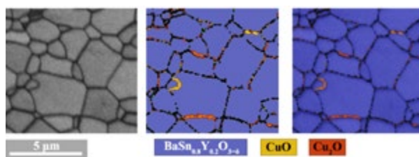
Fig. 1. SEM and EBSD analysis for the BSY-Cu ceramic.
