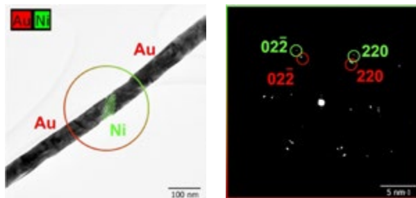
Fig. 1. TEM image of a single Au/Ni/Au nanowire and electron diffraction pattern from a highlighted area containing a thin ferromagnetic nickel layer between gold segments.
