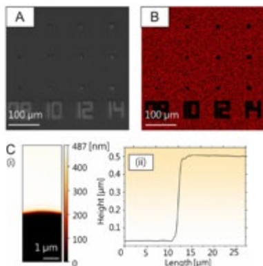
Figure 1. Microscopic characterization of the omniphobic GPOSS-PDMS patterns.
