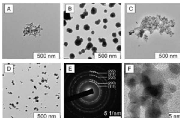
Fig. 1 – TEM images of primary Pt nanoparticles synthesized in gas discharge (a, c) with subsequent sintering at 985°C (b, d) using gas flow rates of 50 and 600 ml/min respectively; diffraction pattern (e) and high-resolution image (f)
