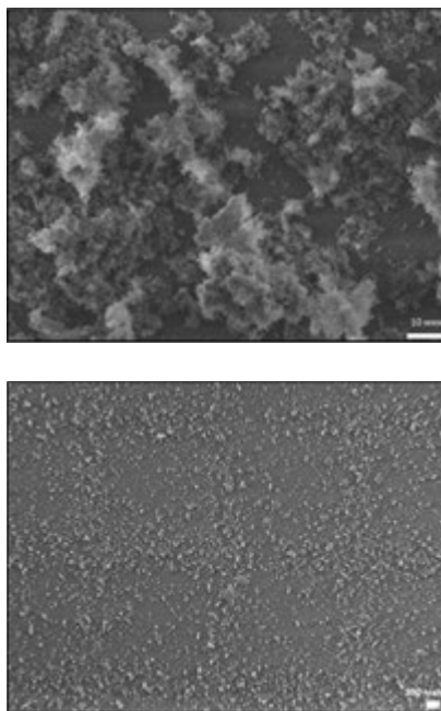
Figure 1. SEM images of aluminum nanostructures (pattern – grid).
